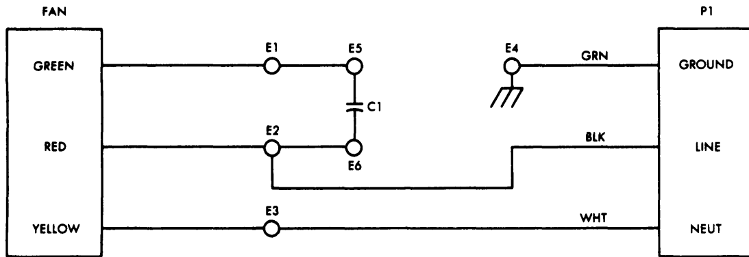
WIRING DIAGRAM
